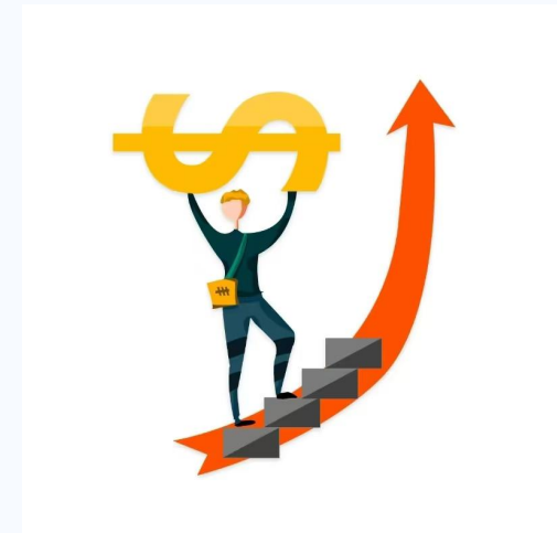
Data analysis
